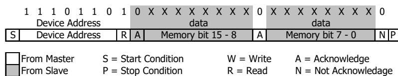
Figure 4: I 2 C answer from MS5837-30BA
