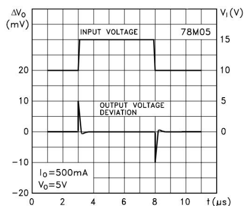
Figure 15. Line transient response
