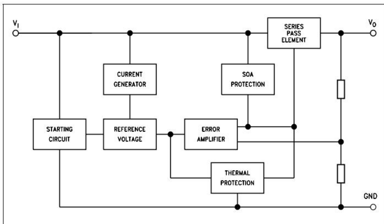
Figure 1. Block diagram
