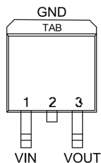
TO-252-2
