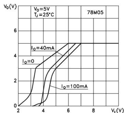
Figure 9. Dropout characteristics
